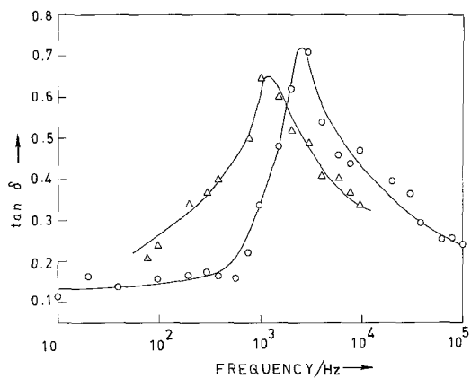
Fig. 8. Dependence of \tan \delta on log of frequency as computed for 130 Å thick oxide film: ○-○ For Al/aluminium oxide/0.5 mol dm -3 ammonium tartrate; △-△ for Al/aluminium oxide/1 mol dm -3 sodium sulphate.
