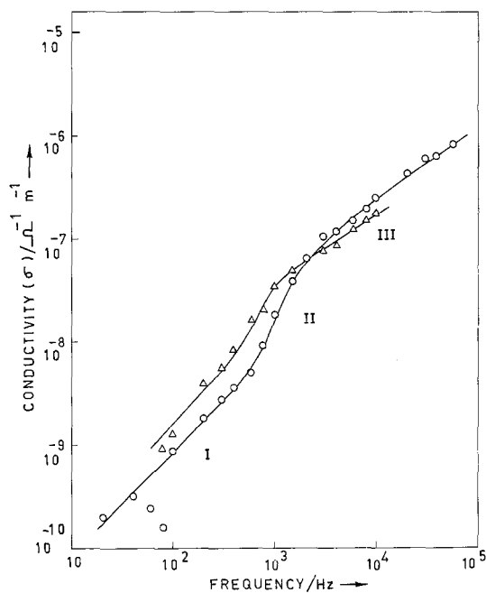
Fig. 9. Dependence of conductivity, \sigma , on frequency as computed for 130 Å thick oxide film: ○-○ For Al/aluminium oxide/0.5 mol dm -3 ammonium tartrate; △-△ for Al/aluminium oxide 1 mol dm -3 sodium sulphate.
